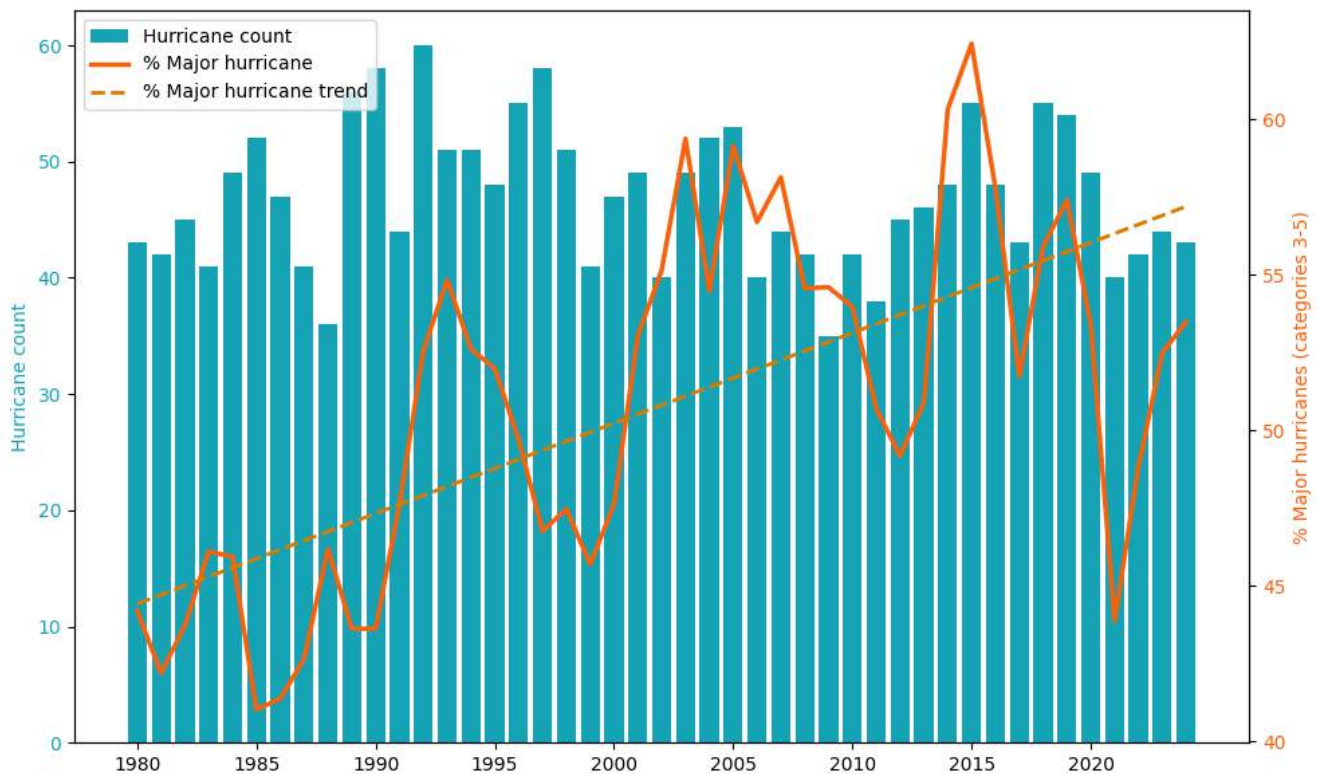
Data as of August 2025, based on the International Best Track Archive for Climate Stewardship project. The light-blue bars show the total number of hurricanes each year (left y-axis), while the orange line shows the share of major hurricanes as a three-year rolling average (right y-axis), smoothing out interannual volatility. The trend highlights the increasing prevalence of more intense hurricanes over time. Source: MSCI ESG Research
