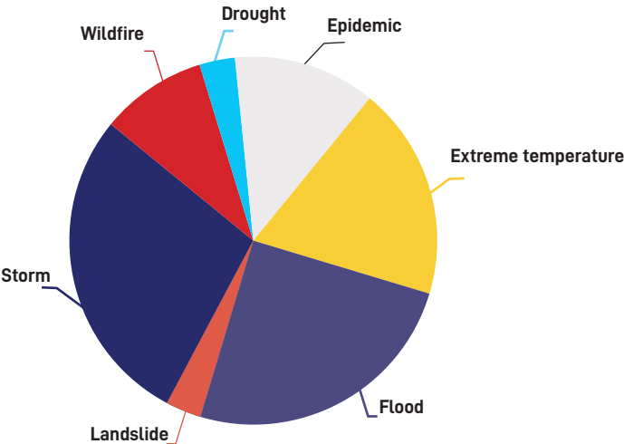
Figure 3. Average Annual Natural Hazard Occurrence for 1980-2020
